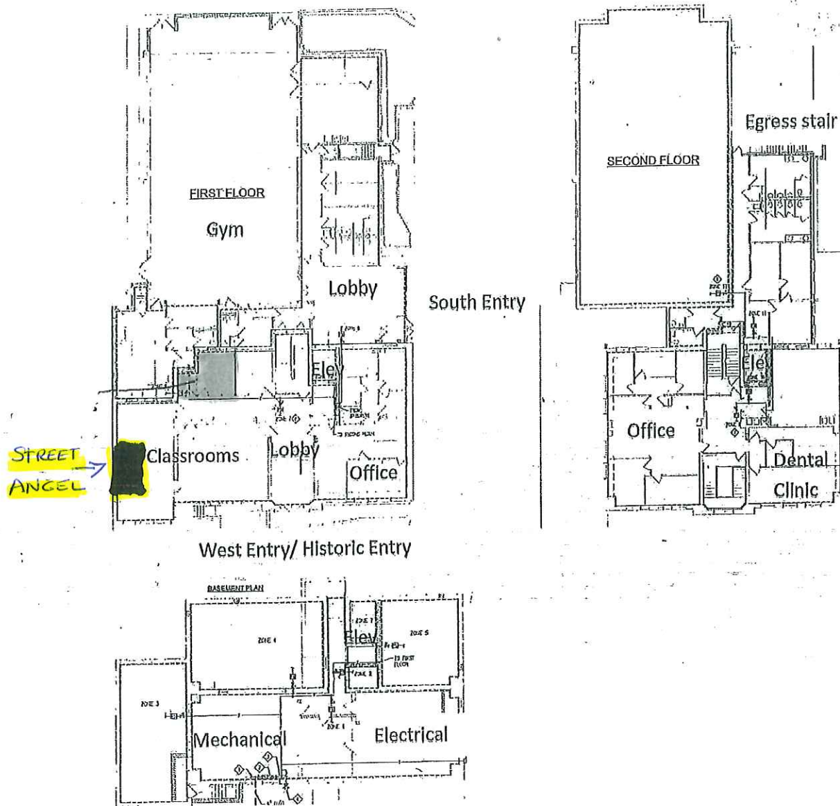
Figure 1-8 Floor Plans
