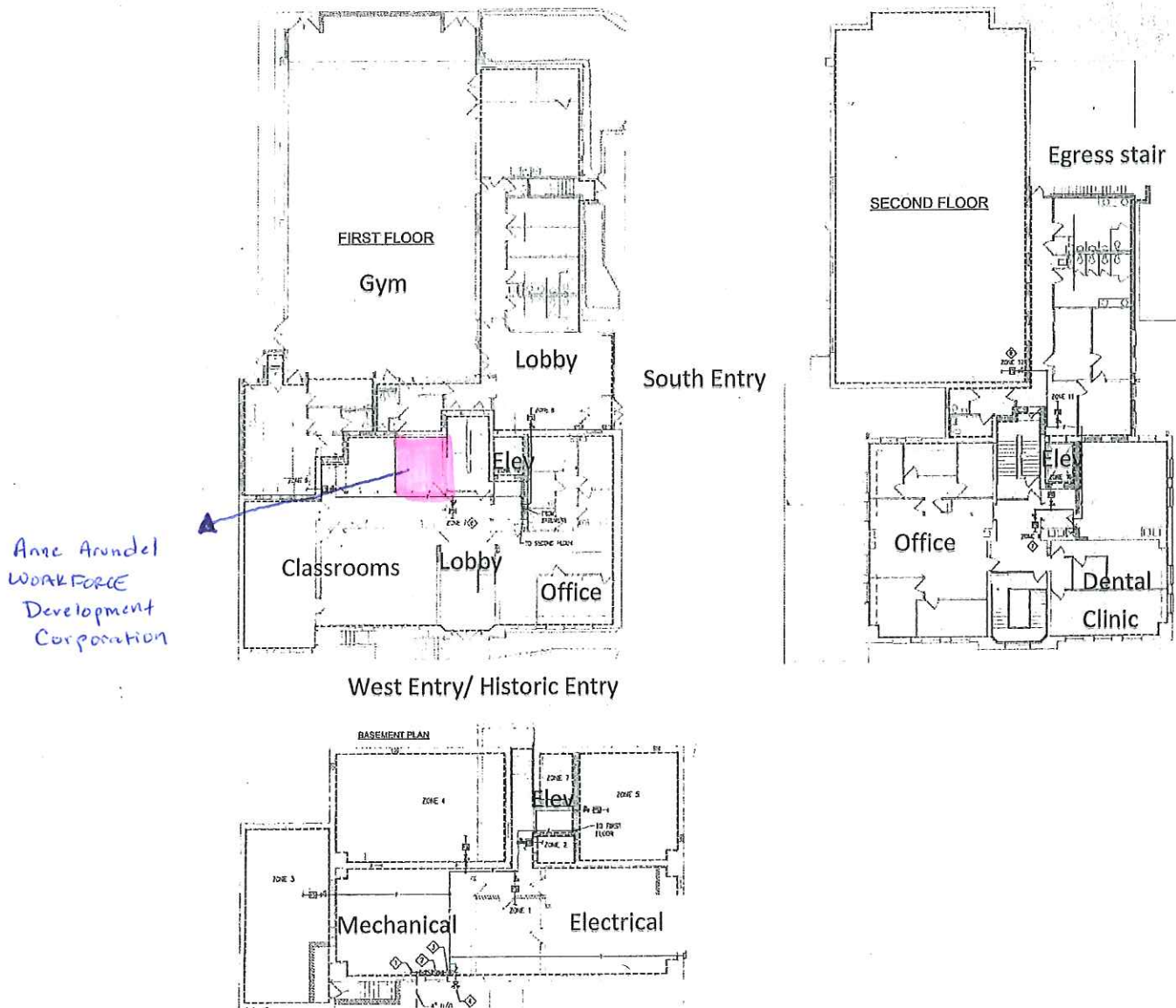
Figure 1-8 Floor Plans
