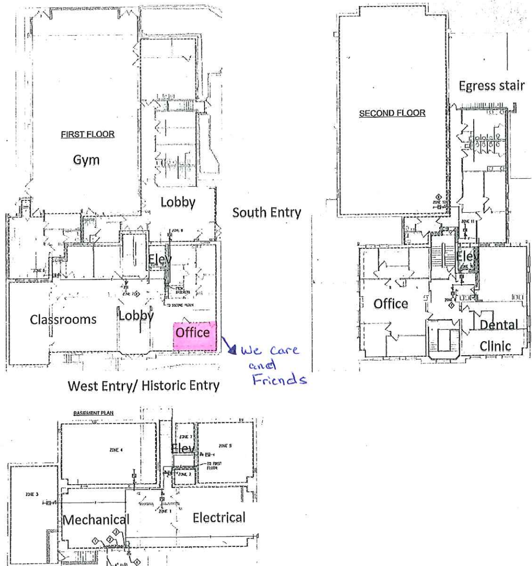
Figure 1-8 Floor Plans
